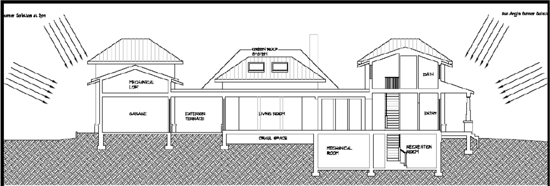
EAST - WEST BUILDING & SITE SECTION
